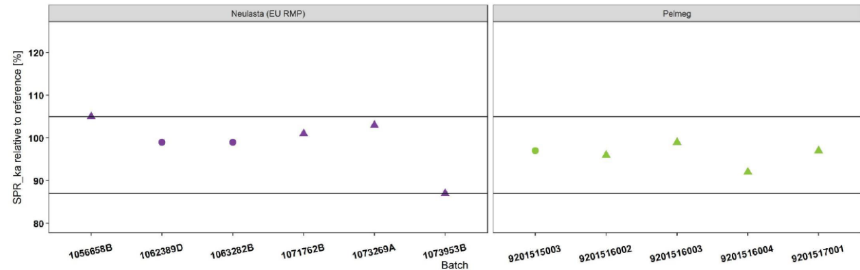
Figure 3: Comparison of SPR ka vales (relative to reference) for Pegfilgrastim Mundipharma and ref. medicinal product batches
