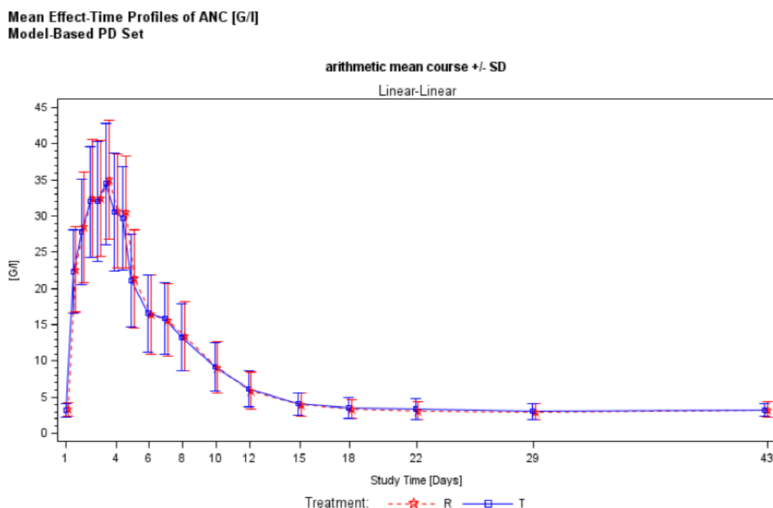
Figure 7: Mean ANC values in Study B12019-101 (Model-based PD set)
