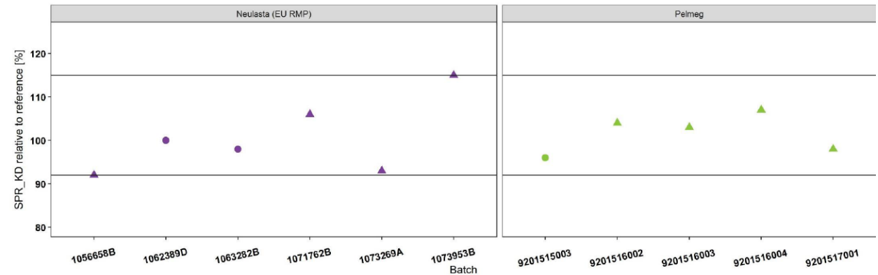
Figure 2: Comparison of SPR KD values (relative to reference) for Pegfilgrastim Mundipharma vs reference medicinal product
