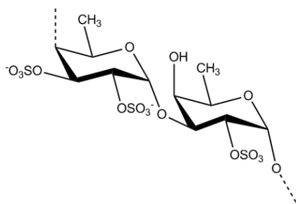
Figure 1: Fucoidan (site glycomix)
