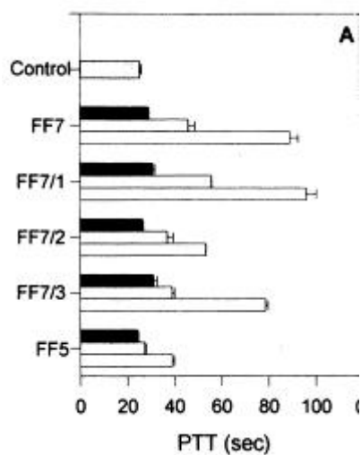
Figure 3: Activated partial thromboplastin time of fucoidan from Fucus vesiculosus (Dürig et al. 1997)
