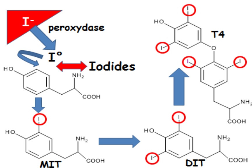
Figure 2: Iodine is transported from the blood compartment to the thyroid gland, to be reduced by peroxidase and subsequently incorporated into the amino acid tyrosine. This process is inhibited by iodides. Mono-iodothyroxine (MIT) and di-iodothyroxine (DIT) are formed. Two units of DIT are fused to tetra-iodothyroxine (T4) or thyroxine (Katzung 2004, DiPiro et al. 2005).
