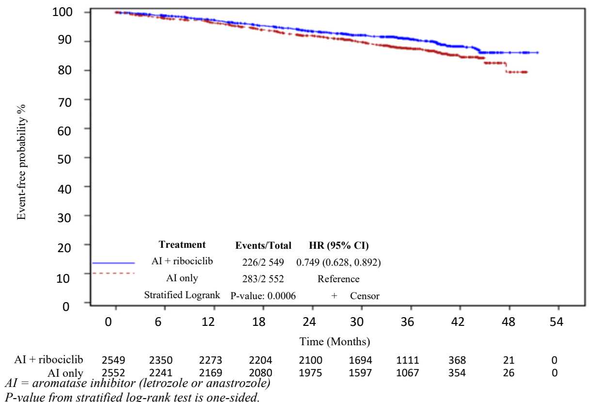
Figure 1 NATALEE - Kaplan-Meier plot of iDFS based on investigator assessment (21 July 2023 cut-off)
