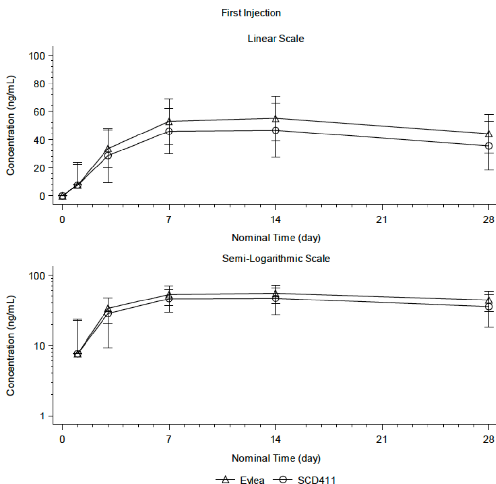
Figure 2. Mean ( \pm SD) bound plasma concentration versus time profiles for SCD411 and Eylea
