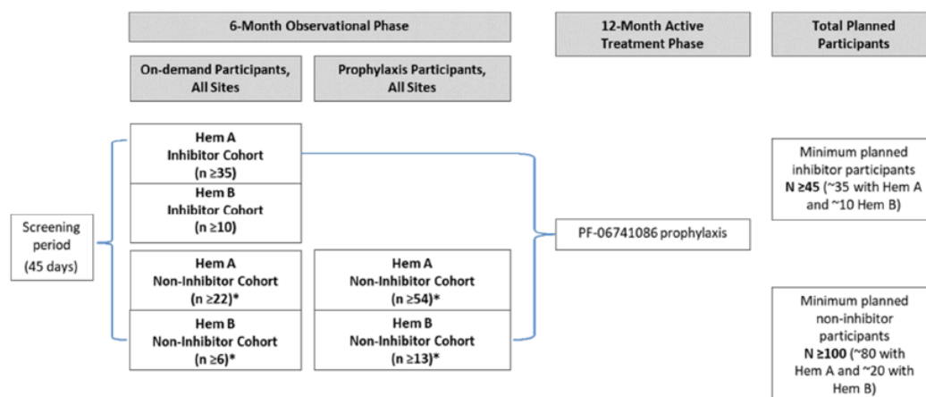
Figure 22: Study schema
