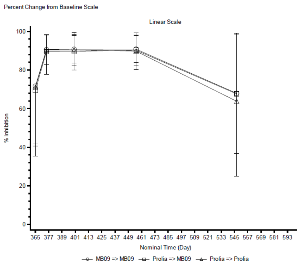
Figure 9: Mean ( \pm SD) percent change from baseline sCTX concentrations versus time following SC administration (linear scale) – Transition period (modified full analysis set for transition period)
