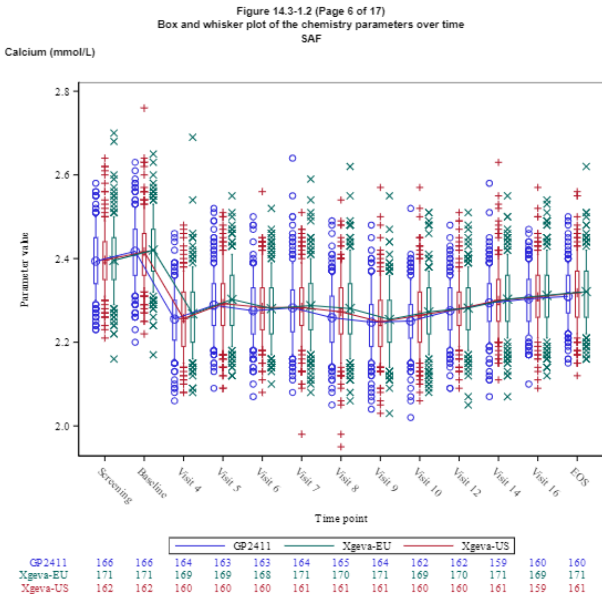
Figure 10. Calcium levels over time (Study CGP24112101, SAF)
