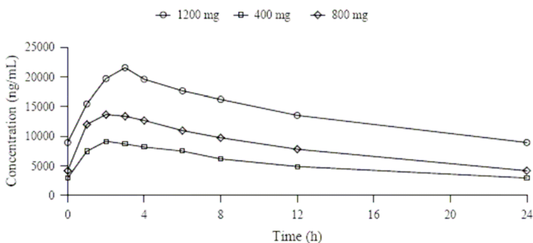
Figure A. Mean eslicarbazepine (BIA 2-194) plasma concentration-time profiles following multiple oral doses of ESL 400 mg, 800 mg and 1200 mg QD
