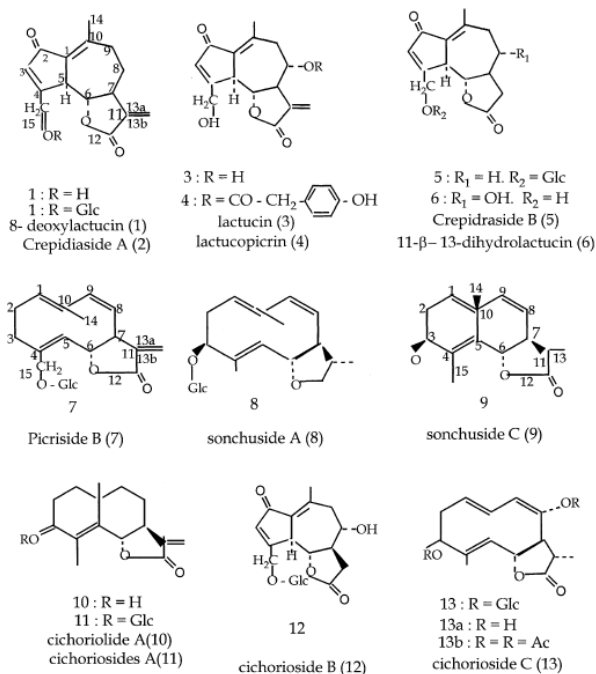
Figure 1. Sesquiterpene lactones isolated from Cichorium intybus (Bais and Ravishankar 2001)
