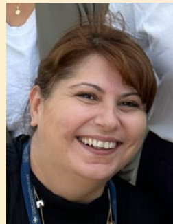
Zhenya Shtereva
