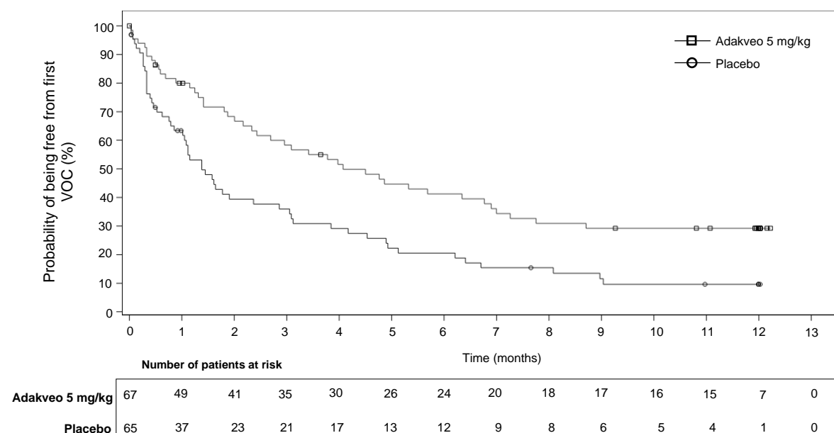
Figure 1 Kaplan-Meier curve of time to first VOC
