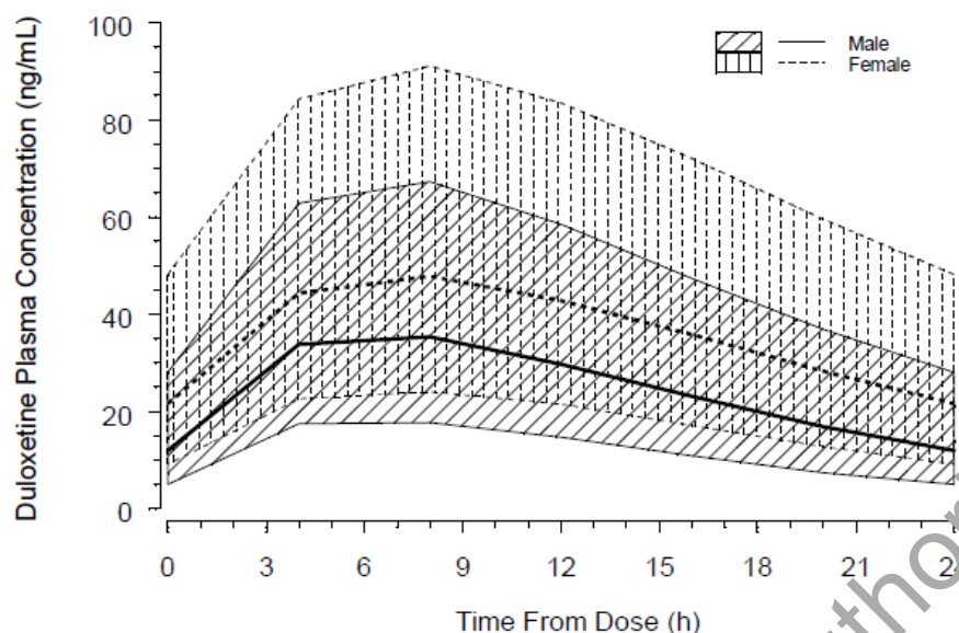
Figure HMFN.11.3. Predicted duloxetine plasma concentration-time profile during the steady state dosing interval of 24 hours following once-daily oral administration of 60 mg duloxetine. Concentrations were simulated for 1000 patients.
