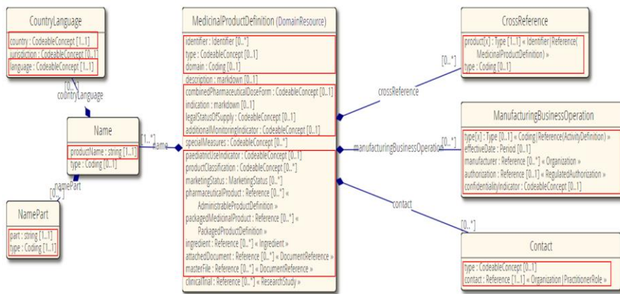
Figure 3: FHIR Resource MedicinalProductDefinition (source: http://www.hl7.org/fhir/ )
