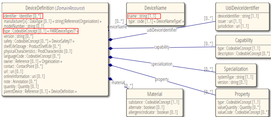
Figure 28: Resource DeviceDefinition (Source : http://www.hl7.org/fhir/ )
