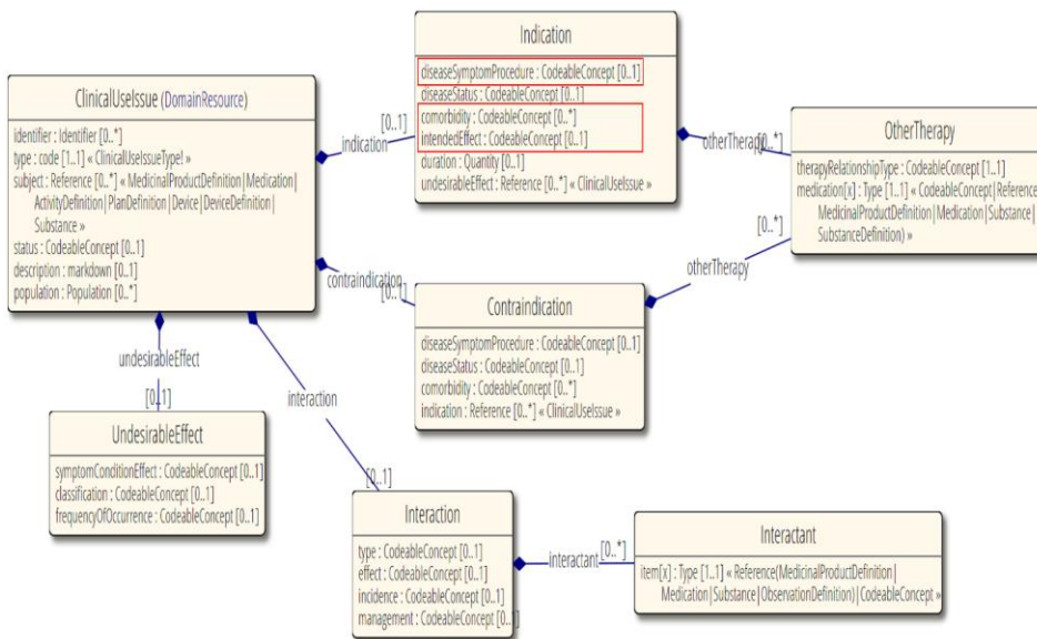
Figure 18: Resource ClinicalUseIssue (source : http://www.hl7.org/fhir )
