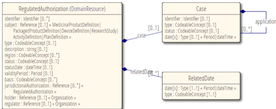
Figure 27: Resource RegulatedAuthorization (source: http://www.hl7.org/fhir )
