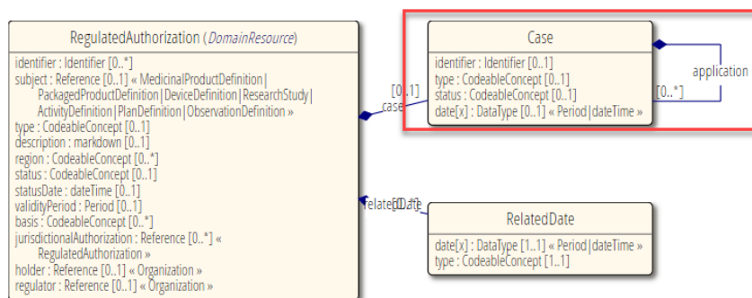
Figure 17: Extract of the Marketing authorization procedure class (source: http://www.hl7.org/fhir )
