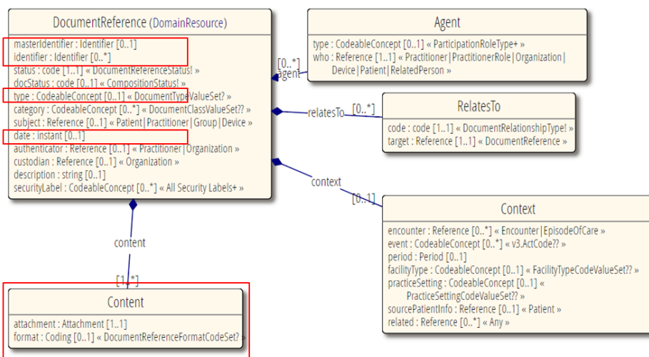
Figure 13: Resource DocumentReference (source : http://www.hl7.org/fhir )
