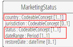
Figure 26: Marketing Status (source: http://www.hl7.org/fhir )
