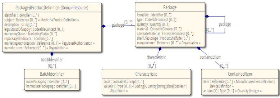
Figure 25: FHIR Resource: PackagedProductDefinition (Source: www.hl7.org/fhir )
