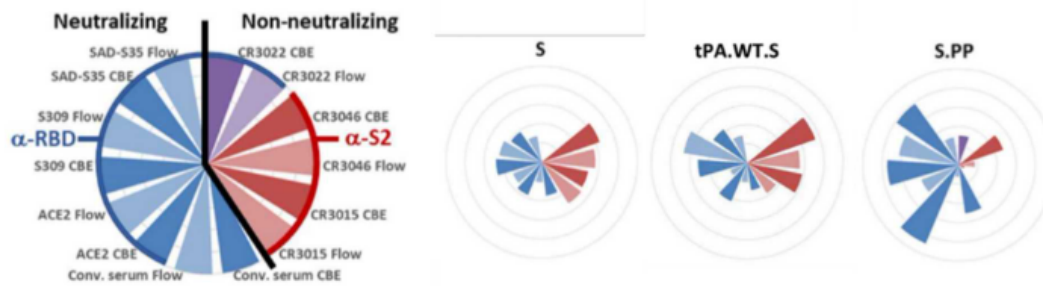
Figure 2: Radar plots showing luminescence intensities measured with cell-based ELISA (CBE) and median fluorescence intensity (MFI) measured with flow cytometry (“Flow”).
